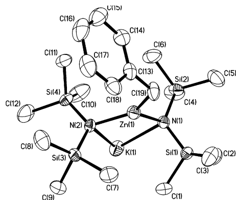
Fig. 1 Asymmetric unit of the structure of 1 with atom labels and 50% probability displacement ellipsoids. Hydrogen atoms have been omitted for clarity. Key dimensions not in text (Å and °): N–Si; 1.703(4)–1.724(4); N(1)–K(1)–N(2) 72.82(9), N(1)–Zn(1)–N(2) 114.06(13), N(1)–Zn(1)–C(19) 115.59(15), N(2)–Zn(1)–C(19) 130.30(15), Zn(1)–C(19)–C(13) 117.0(3).
