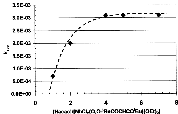
Fig. 3. Plot of k app (s −1 ) vs. [Hacac]/[ 5 ], in experiment 1.
