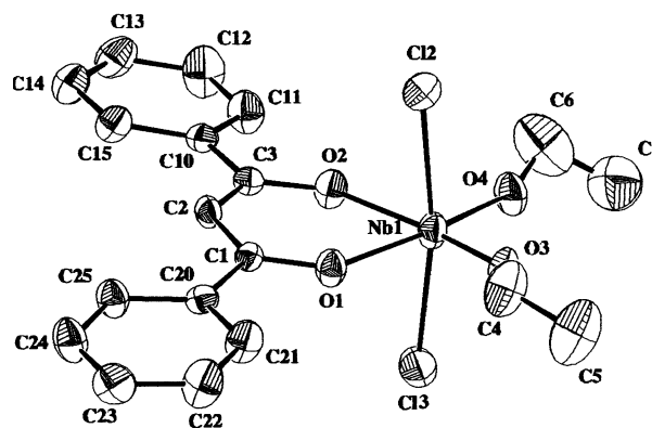
Fig. 2. ORTEP drawing of complex 8.
