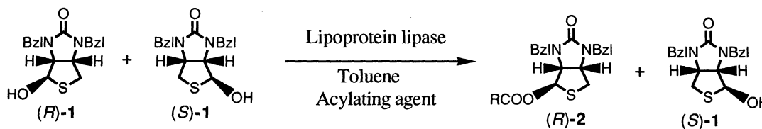
Scheme 1. Lipoprotein lipase-catalyzed acylation.
