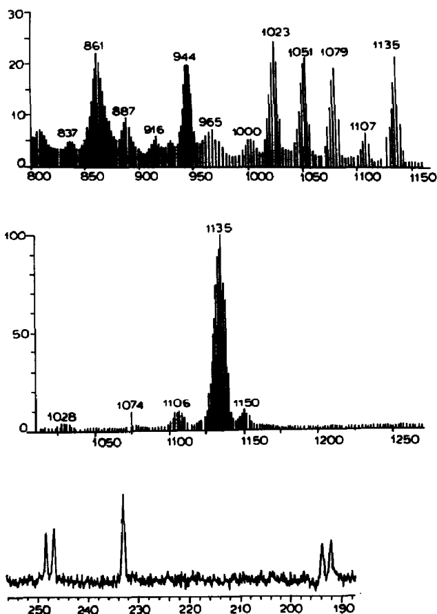
Fig. 4. Positive and negative ion FAB mass spectra (top and bottom, respectively) and ^{31}\text{P} NMR spectrum of complex 9.
