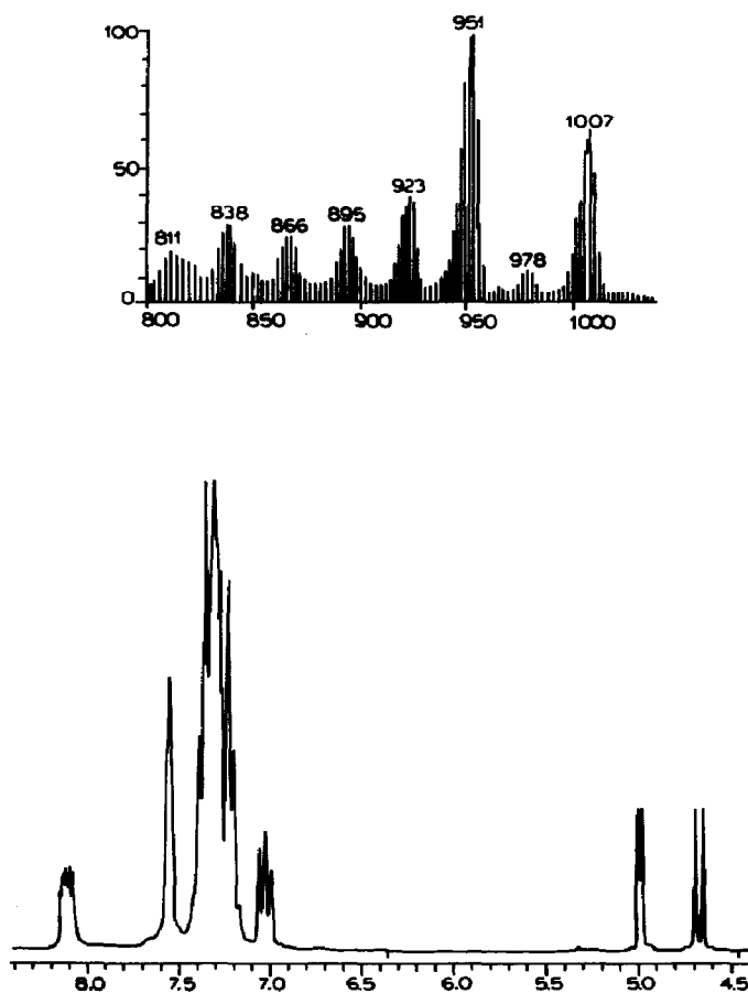
Fig. 2. FAB mass spectrum and ^1\text{H} NMR spectrum of complex 8 .
