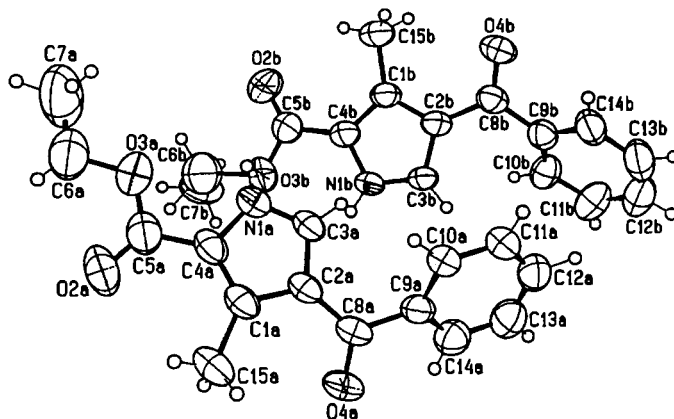
Figure 3. Ortep view of two molecules that compose asymmetric unit of 9 with labeling of nonhydrogen atoms. (Ellipsoids are drawn at 40% probability level.)
