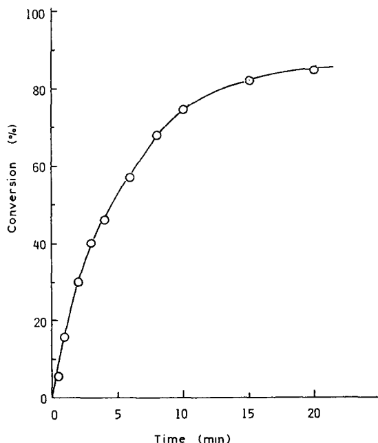
Fig. 1. Typical conversion curve of hydrogenation of cyclohexanone catalyzed by [\text{Rh}((i\text{-Pr})_2(\text{CH}_2)_4\text{P}(i\text{-Pr})_2)(\text{NBD})]\text{ClO}_4 ; [\text{Rh}] = 0.5 \text{ mM} ; [\text{ketone}]_0 = 0.1 \text{ M} ; [\text{H}_2] = 1.0 \text{ atm} ; in MeOH at 35^\circ\text{C} .
