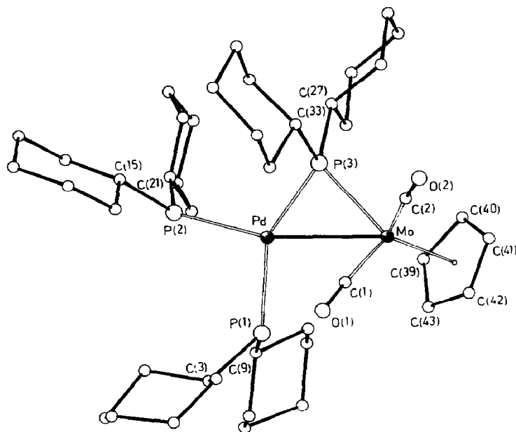
Fig. 1. View of the molecular structure of (\eta\text{-C}_5\text{H}_5)(\text{CO})_2\text{Mo}(\mu\text{-PCy}_2)\text{Pd}(\text{PCy}_2\text{H})_2 ( 2a ). The H atom bound to P(1) and P(2) is not shown. Selected bond distances (Å) and angles ( ^\circ ): Pd–Mo 2.916(2), Pd–P(1) 2.362(4), Pd–P(2) 2.380(5), Pd–P(3) 2.278(4), Mo–P(3) 2.367(3); Mo–Pd–P(1) 97.1(1), Mo–Pd–P(3) 52.5(1), P(1)–Pd–P(2) 96.7(2), P(2)–Pd–P(3) 113.7(2), Pd–P(3)–Mo 77.7(1).
