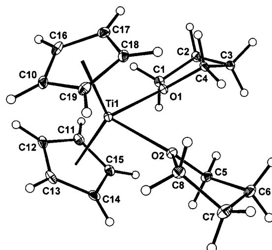
Figure 2. Molecular structure of the cation in [Cp 2 Ti(THF) 2 ][HB(C 6 F 5 ) 3 ], 3 , showing 15% probability thermal ellipsoids. Hydrogens attached to carbon atoms are shown with arbitrary thermal ellipsoids.
