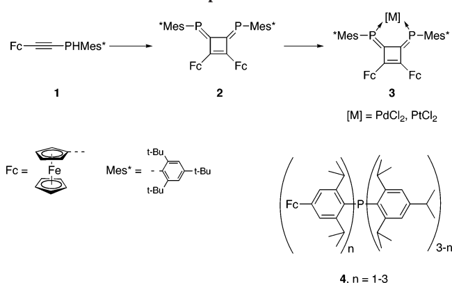
Scheme 1. Redox-Active, Ferrocenyl-Functionalized Phosphanes 17,18
