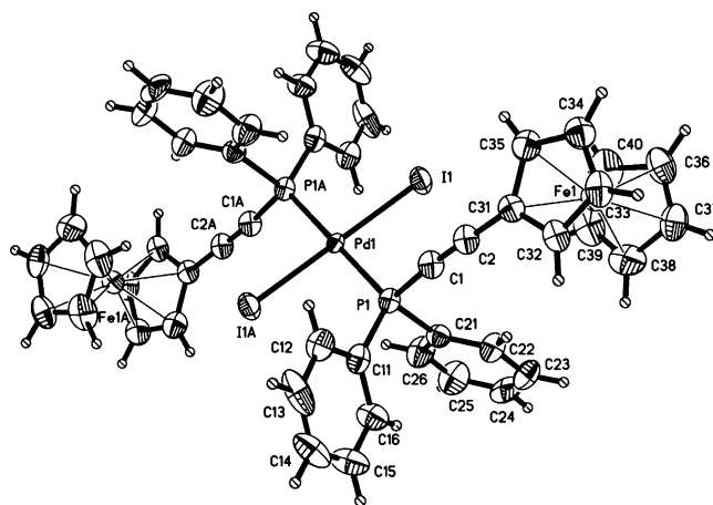
Figure 3. Molecular structure of 13 in the solid state (50% probability level). Selected bonds lengths (Å) and angles (deg): Pd1–P1: 2.314(3); P1–C1: 1.736(12); C1–C2: 1.199(18); C2–C3: 1.420(17); I1–Pd1–I1A: 180.00(4); P1–Pd1–P1A: 180.0; P1–Pd1–I1: 87.67(8); P1A–Pd1–I1: 92.33(8); Pd1–P1–C1: 114.6(5); P1–C1–C2: 172.4(12); C1–C2–C3: 177.1(13).
