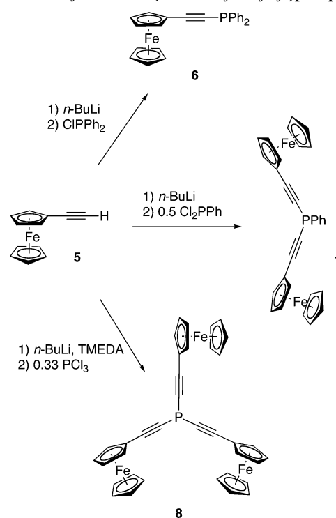
Scheme 2. Synthesis of (Ferrocenylethynyl)phosphanes
