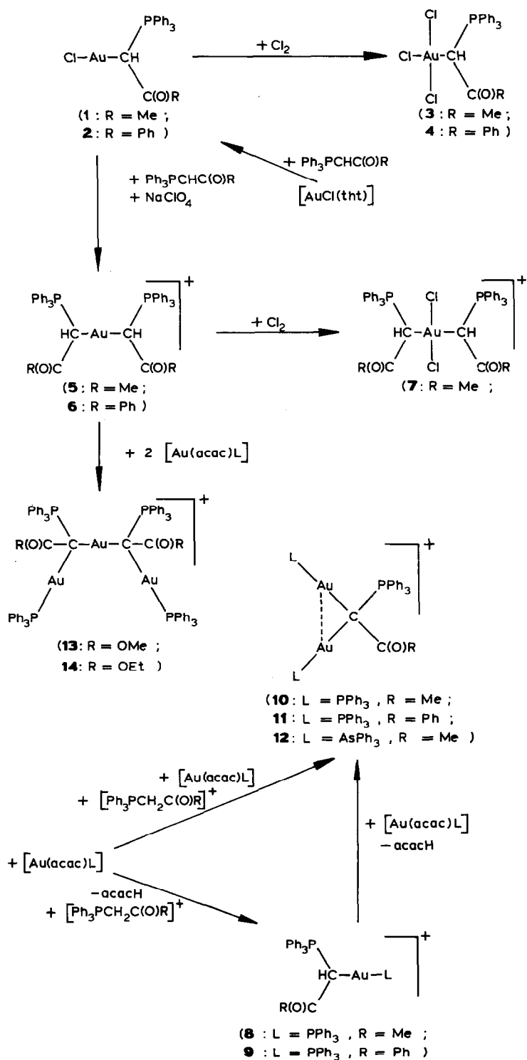
Scheme 1. Synthesis of complexes 1-14.
