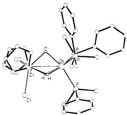
Figure 1. ORTEP drawing of one molecule of \text{Cp}_2\text{ZrClZrH}_3\text{Os}(\text{PMe}_2\text{Ph})_3 . Presumed hydride bridge locations have been added, trans to Os-P bonds, using \text{M}-(\mu_2\text{-H}) distances from [(\text{C}_5\text{H}_4\text{Me})_2\text{ZrH}_2]_2^{21} and \text{H}_2\text{Os}_3(\text{C}-\text{O})_{10} . 22 Unlabeled atoms represent carbon. Selected structural parameters: Os-Zr 2.805 (1), Os-P 2.300 (3)–2.330 (3), Zr-Cl 2.521 (3) Å; \angle\text{Zr-Os-P} 117.7 (1)–123.4 (1)°, \angle\text{P-Os-P} 94.1 (1)–100.8 (1)°, \angle\text{Cl-Zr-Os} 98.6(1)–98.9 (1)°.
