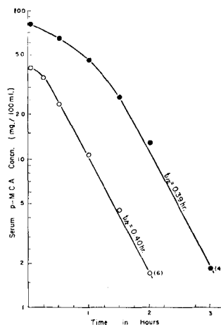
Fig. 2—Elimination of p -MCA from serum following its intravenous injection of 100 mg./Kg. (○) and 200 mg./Kg. (●). Figure in parentheses at the right of each line is number of rabbits used.
