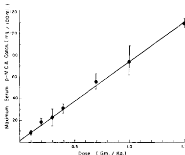
Fig. 4—Linear relationship between mean maximum serum concentration of p -MCA and oral dose.
