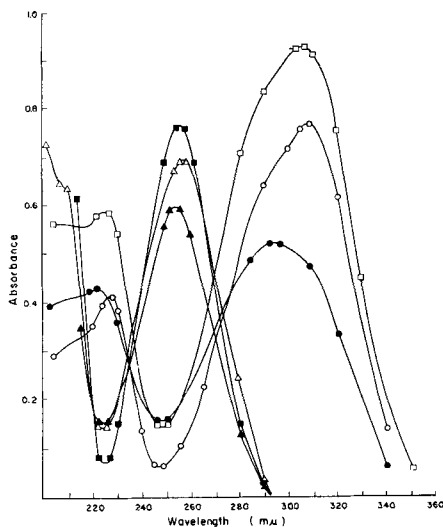
Fig. 6—UV absorption spectra of p -MCA and its related compounds in 5% HClO 4 . Key: ○, p -MCA (8.3 mcg./ml.); ●, p -MCG (8.8 mcg./ml.); □, p -HCA (9.6 mcg./ml.); ■, p -HBA (8.0 mcg./ml.); △, p -MBA (8.0 mcg./ml.); ▲, p -MBG (8.0 mcg./ml.).
