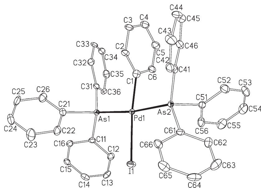
Fig. 2. Thermal ellipsoid plot (50% probability) of catalysis intermediate \text{trans-[Pd}^{\text{II}}(\text{I})(\text{Ph})(\text{AsPh}_3)_2] ( 7 ). H-Atoms are omitted for clarity; for selected bond distances and angles, see Table 2.
