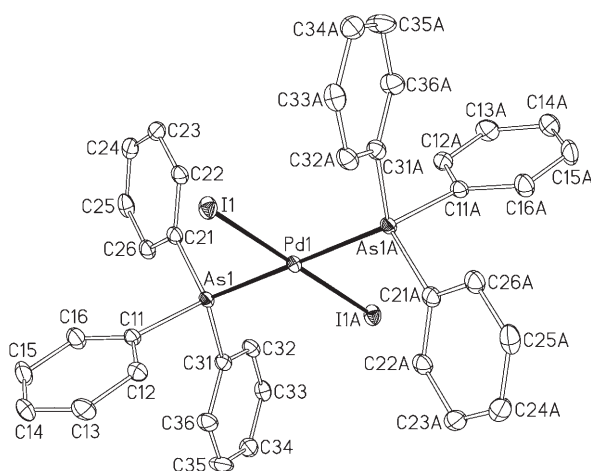
Fig. 3. Thermal ellipsoid plot (50% probability) of \text{trans-[Pd}^{\text{II}}(\text{I})_2(\text{AsPh}_3)_2] ( 8 ). H-Atoms are omitted for clarity; for selected bond distances and angles, see Table 3.
