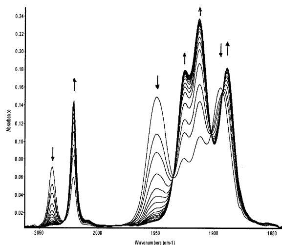
Fig. 1. The FT-IR spectra taken in the course of the thermal substitution reaction of 2A with DPPM at 20^\circ\text{C} with a time interval of ca. 20 min. [\text{DPPM}]_0/[\text{2A}]_0 = 10 .
