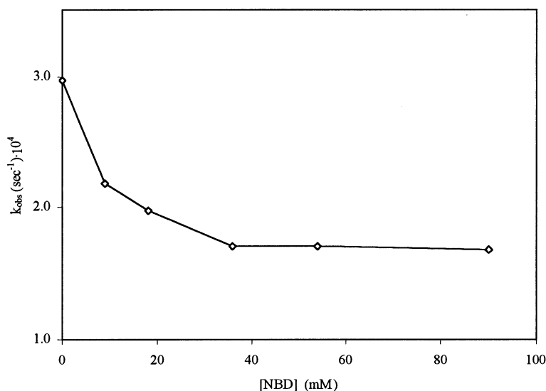
Fig. 4. Variations in the observed rate constants ( k_{\text{obs}} ) with the concentration of NBD for the substitution of NBD in 1A with DPPE at 85°C. [\text{1A}]_0 = [\text{DPPE}]_0 = 9.00 \text{ Mm} .
