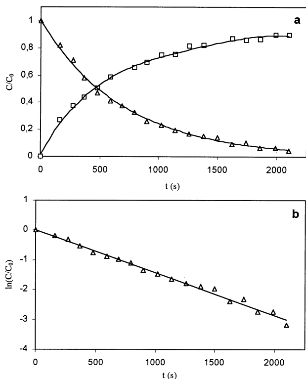
Fig. 2. (a) The normalized concentration vs. time plot for the substitution reaction of 2A ( \Delta ) with DPPM at 15°C forming 2B ( \square ), [PP]_0/[2B]_0 = 10 ; (b) plot of the first-order kinetics for the same reaction.
