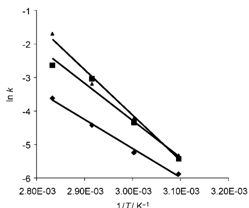
Figure 4. Arrhenius plots for the racemization of ( R )-1-phenylethanol over acid catalysts under standard conditions. Catalysts: Amberlyst ® 15 ( \blacklozenge ), H-Beta ( \blacksquare ), and 0.5 M p TSA ( \blacktriangle ).
