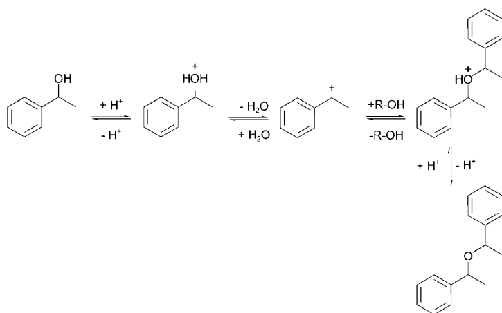
Scheme 2. Formation of 1-phenylethyl ether as a potential side reaction.
