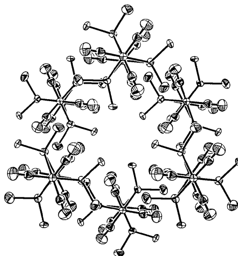
Fig. 2. Packing diagram of (I). Displacement ellipsoids are drawn at the 50% probability level.
