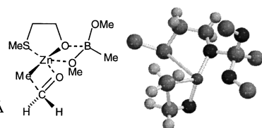
Figure 1. Calculated transition structure forming ethanol by methylation of formaldehyde. Some hydrogens have been omitted for clarity.
