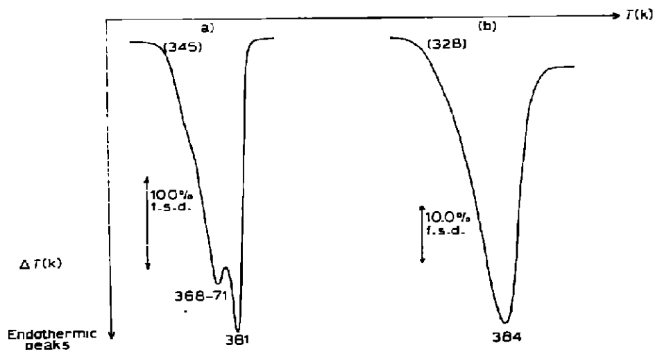
Fig. 4. DTA curves for strontium formate dihydrate (50 mg samples diluted with 40 mg alumina reference material). Heating rate 10\text{ K min}^{-1} ; 100\text{ }\mu\text{V f.s.d.} (a) 500\text{ cm}^3\text{ min}^{-1} nitrogen, (b) reduced pressure (ca. 0.25 mm Hg).
