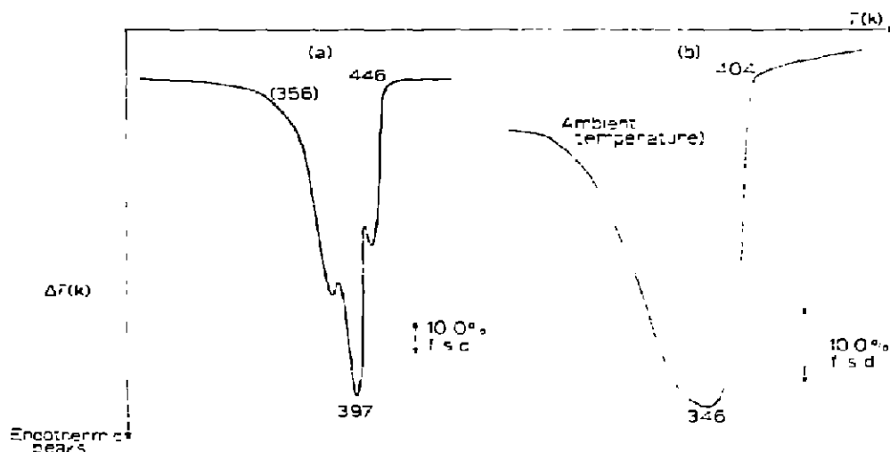
Fig. 1. DTA curves for strontium hydroxide octahydrate. Heating rate 10 \text{ K min}^{-1} ; 100 \mu\text{V f.s.d.} (a) 80 mg sample, 300 \text{ cm}^3 \text{ min}^{-1} nitrogen, (b) 60 mg sample, continuously evacuated. Temperatures in parentheses are extrapolated onset temperatures. All other temperatures are either peak temperatures or temperatures at which peaks terminate.
