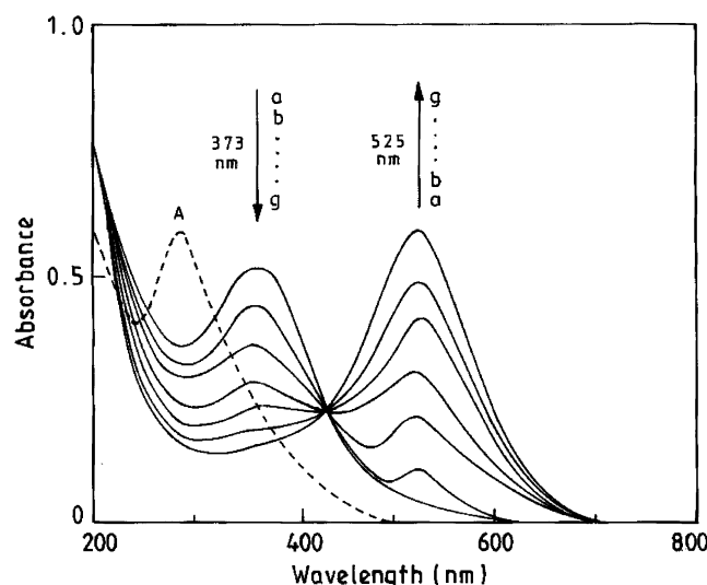
Figure 1. Successive evolution of plasmon bands for isotropic Au particles generated from Au(III)-Acac chelate. The dotted line with a peak at 290 nm displays the absorption spectrum of aqueous \text{HAuCl}_4 solution indicating a metal to ligand charge-transfer (MLCT) band. The concomitant decrease of the absorbance value at 373 nm was attributed to the decomposition of the Au(III)-Acac complex with time (a-f, 2–30 min). The successive increase of the plasmon band at 525 nm with time (a-f, 2–30 min) stands for the formation of Au nanoparticles.
