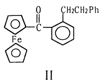
Fig. 1. The structural formulas for compounds I–IV.
