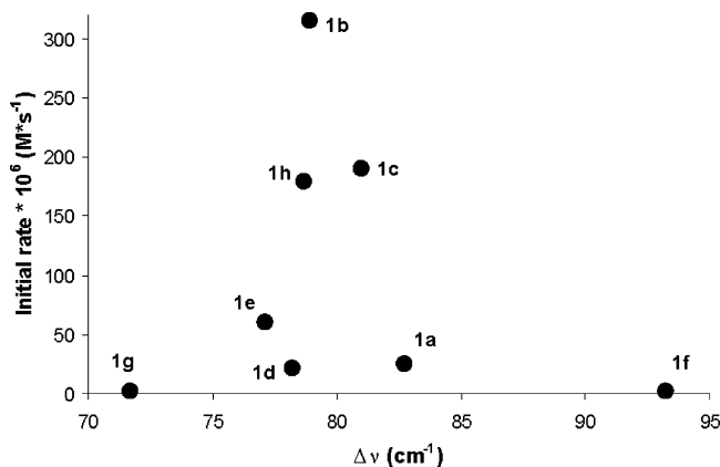
Figure 2. Plot of the initial rates of epoxidation of 1-octene catalyzed by complexes 1a–h vs the \Delta\nu values (cm -1 ) of 2,6-dimethyl phenylisocyanide coordinated to the complexes 1a–h . Experimental conditions as in Table 2.
