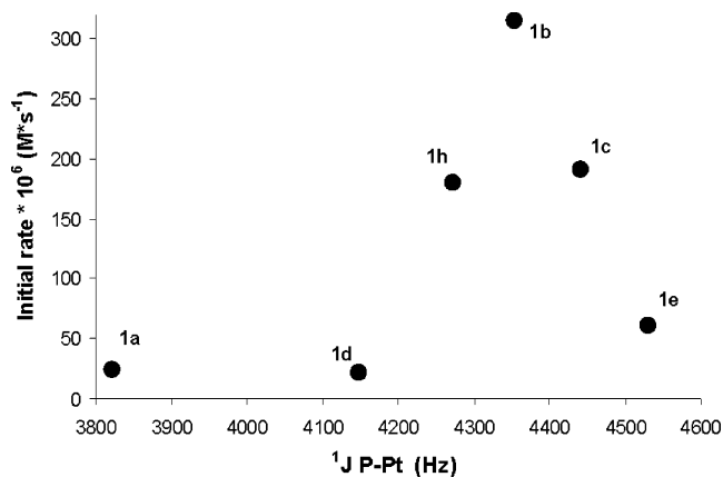
Figure 3. Plot of the initial rates of epoxidation of 1-octene catalyzed by complexes 1a–h vs the ^1J_{P-Pt} (Hz) trans to the water ligand of the complexes. Experimental conditions as in Table 2.
