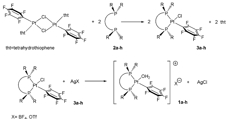
Scheme 2. Synthesis of the Pt(II) Monocationic Catalysts 1a–h Bearing a Perfluorophenyl Residue
