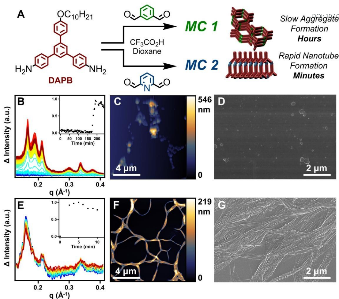
Figure 2. Probing the kinetics of the assembly processes that govern the formation of MC 1 and MC 2 . (A) Scheme of macrocycle formation. (B) TR-XRD patterns from 0 to 240 minutes depicting the formation and assembly of MC 1 . (Inset) Normalized integration of the diffraction signal with respect to time. (C) Atomic force micrograph of the aggregates resulting from the formation of MC 1 . (D) Scanning electron micrograph of the aggregates resulting from the formation of MC 1 . (E) TR-XRD patterns from 0 to 10 minutes depicting the rapid formation and assembly of MC 2 . Slight decreases in intensity were observed due to x-ray beam damage of the resulting nanotubes. (Inset) Normalized integrations of the diffraction signal with respect to time. (F) Atomic force micrograph of the nanotubes resulting from the formation of MC 2 . (G) Scanning electron micrograph of the nanotubes resulting from the formation of MC 2 .
