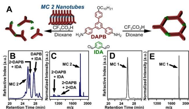
Figure 4. Control experiment demonstrating the effects of MC 2 nanotubes on the selective synthesis of MC 1 . (A) Scheme depicting the control experiment in which previously synthesized MC 2 nanotubes are combined with DAPB, IDA, and CF 3 CO 2 H under conditions which in the absence of MC 2 nanotubes selectively yields MC 1 . (B) Gel permeation chromatogram of the inhibited MC 1 synthesis. (C) MALDI-MS spectra of the results of the inhibited MC 1 synthesis depicting the recovery of MC 2 , with no hydrolysis artifacts, and oligomers containing IDA moieties. MC 2 was observed as the [M+H]^+ , [M+Na]^+ , and [M+K]^+ adducts. (D) Representative gel permeation chromatogram of the direct synthesis of MC 1 . (E) Representative MALDI-MS spectra of the direct synthesis of MC 1 .
