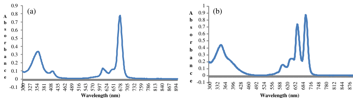
Figure 1. UV-vis spectra of phthalocyanines 7 (a) and 8 (b) recorded in \text{CH}_2\text{Cl}_2 .
