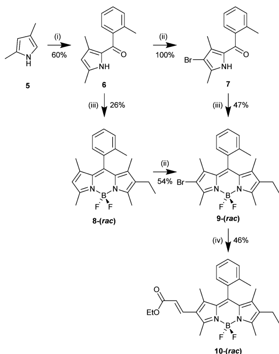
Scheme 1 Synthesis of 10-(rac) . (i) (a) EtMgBr, Et 2 O, reflux, 1 h (b) 2-methylbenzoyl chloride, rt, 24 h (ii) Br 2 , DCM, rt, 24 h (iii) (a) 2,4-dimethyl-3-ethylpyrrole, TFA, DCM, rt, 18 h (b) i -Pr 2 NEt, BF 3 OEt 2 , rt, 12 h (iv) ethyl acrylate, Et 3 N, Pd(OAc) 2 , PPh 3 , DMF, 100 °C, 12 h.
