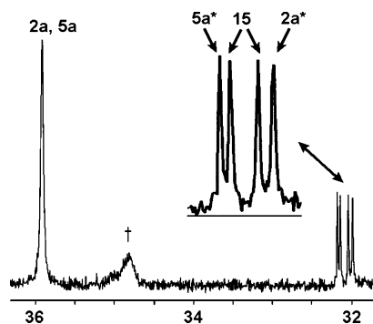
Figure 7. ^{31}\text{P} NMR spectrum (162 MHz, \text{CD}_2\text{Cl}_2 , 25 ^\circ\text{C} ) of an equilibrium mixture of macrocycles and [2]catenanes 2a/2a* ( \text{X} = \text{X}' = \text{CMe}_2 ) and 5a/5a* ( \text{X} = \text{X}' = \text{C}_6\text{H}_{10} ) to give the mixed ligand [2]catenane 15 ( \text{X} = \text{CMe}_2 , \text{X}' = \text{C}_6\text{H}_{10} ). The broad peaks marked \dagger are assigned to the double ring and hexamer isomers.
