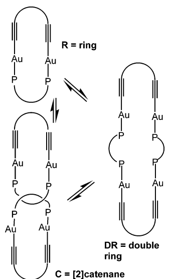
Scheme 1. Equilibrium between Ring, Double Ring, and [2]Catenane
