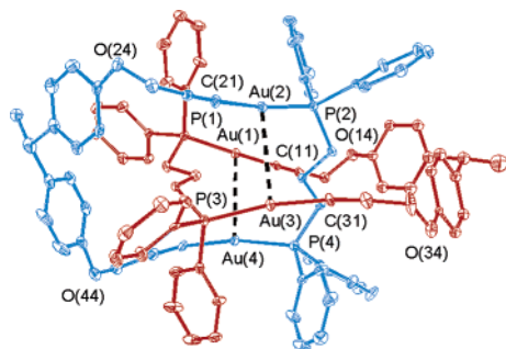
Figure 5. View of the structure of the chiral [2]catenane 7a* ( X = \text{CHMe} , Z = (\text{CH}_2)_3 ). Selected bond distances (Å) and angles (deg): Au(1)–Au(4) 3.3314(4); Au(2)–Au(3) 3.3622(4); Au(1)–P(1) 2.2756(18); Au(2)–P(2) 2.2787(18); Au(3)–P(3) 2.2742(18); Au(4)–P(4) 2.2666(18); Au(1)–C(11) 1.994(8); Au(2)–C(21) 1.989(7); Au(3)–C(31) 1.988(7); Au(4)–C(41) 2.004(7); P(1)–Au(1)–C(11) 174.1(2); P(2)–Au(2)–C(21) 173.3(2); P(3)–Au(3)–C(31) 171.2(2); P(4)–Au(4)–C(41) 168.9(2); Au(1)–C(11)–C(12) 174.1(6); Au(2)–C(21)–C(22) 175.5(7); Au(3)–C(31)–C(32) 172.3(7); Au(4)–C(41)–C(42) 170.5(7); C(11)–C(12)–C(13) 177.5(8); C(21)–C(22)–C(23) 177.7(8); C(31)–C(32)–C(33) 174.8(9); C(41)–C(42)–C(43) 173.2(9).
