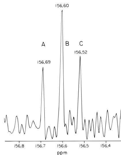
Figure 9. The C _{\alpha} -OL (L = H, D) region in the ^{13}\text{C} NMR spectrum of 25: (A) 25; (B) 25-D; and (C) 25-D _2 . Solvent: 42:5:3 DMF:THF:H _2 O. The spectrum was obtained after 4 h acquisition time.
