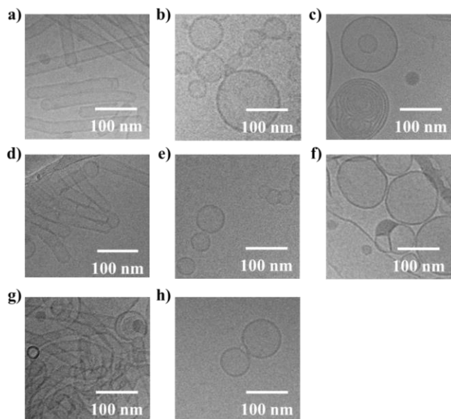
Figure 11. Reversibility of isomerization of co-assemblies of 2 and DOPC (1:1) in water by cryo-TEM at a total concentration
