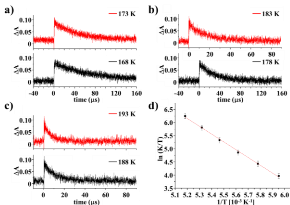
Figure 6. Transient recoveries for 1 (at \lambda = 430 nm, in isopentane) upon pulsed irradiation at \lambda = 355 nm at various temperatures. a) 168 K; 173 K. b) 178 K; 183 K. c) 188 K; 193 K. d) Eyring plot for the thermal helix inversion of unstable 1 to stable 1 .
