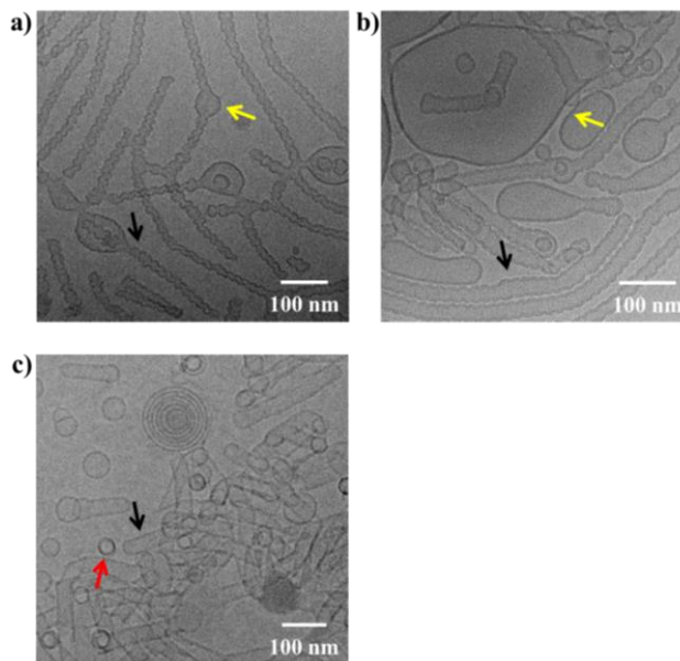
Figure 3. Cryo-TEM microscopy images of a) Co-assemblies of amphiphile 1 and DOPC (ratio 1:1). b) Extruded (pore size 200 nm) co-assemblies of amphiphile 1 and DOPC (ratio 1:1). 71 c) Co-assemblies of amphiphile 2 and DOPC ratio 1:1). 72 Samples are in water and the total concentration of amphiphile is 1 mg/mL. Black arrows indicate nanotubes in the specimen plane; yellow arrows indicate DOPC bilayers;
