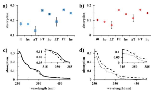
Figure 10. Reversibility of isomerization of co-assemblies of 2 and DOPC (1:1) in water at a total concentration of 1 mg/mL. a) UV-vis absorption maxima at \lambda = 295 nm (blue squares) and b) \lambda = 345 nm (red diamonds). to = starting point; h\nu = sample irradiated for 10 min at \lambda = 365 nm; \Delta T = sample heated at 50 °C for 16 h; FT = sample freeze-thawed 3 times. c) Nanotubes of stable 2 with DOPC (1:1) in water (1 mg/mL) before (solid line) and after (dashed line) irradiation (10 min, \lambda_{\text{irr}} = 365 nm; unstable 2 ), followed by d) heating at 50 °C for 16 h (dashed to dotted line; stable 2 ). The cycles were performed in triplo. Insets are expanded areas of \lambda = 315 –385 nm.
