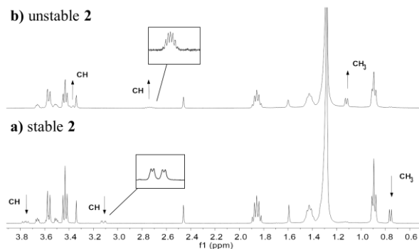
Figure 8. Partial ^1H NMR spectra of a) stable 2 before and b) unstable 2 after irradiation (2 h, \lambda_{irr} = 365 nm) in CH_2Cl_2 at 20 °C.
