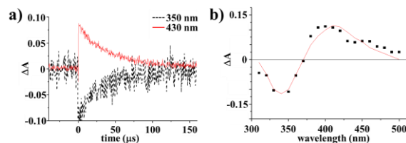
Figure 5. Transient decay and recovery following pulsed excitation of 1 in isopentane at 173 K. a) At \lambda = 350 nm (black striped line) and \lambda = 430 nm (red solid line). b) UV-vis difference spectrum 100 ns after excitation.
