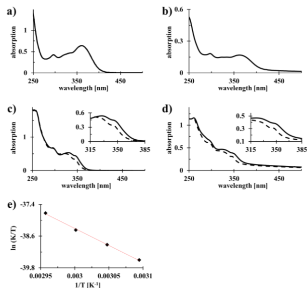
Figure 4. UV-vis absorption spectra. a) Solution of 1 in MeOH ( 2.5 \cdot 10^{-6} M) before and after irradiation (10 min, \lambda_{\text{irr}} = 365 nm). b) Nanotubes of 1 with DOPC (1:1) in water (1 mg/mL) before and after irradiation (10 min, \lambda_{\text{irr}} = 365 nm). c) Solution of 2 in \text{CH}_2\text{Cl}_2 ( 2.5 \cdot 10^{-6} M) before (solid line) and after (dashed line) irradiation (2 h, \lambda_{\text{irr}} = 365 nm). d) Nanotubes of 2 with DOPC (1:1) in water (1 mg/mL) before (solid line) and after (dashed line) irradiation (10 min, \lambda_{\text{irr}} = 365 nm). e) Eyring plot for the thermal helix inversion of unstable 2 to stable 2 . Spectra before and after irradiation in (a) and (b) overlap. Insets in (c) and (d) are expanded areas of \lambda = 315\text{--}385 nm.
