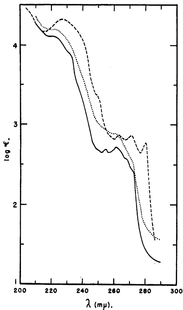
Fig. 1.—Ultraviolet absorption spectra (Cary spectrophotometer, model 11MPS) in cyclohexane: ····, 2,3-diphenyl-2-ethoxyethylenimine (VII); ----, 2,3-bis-(4'-chlorophenyl)-ethylenimine (XI); —, 2,3-diphenylethylenimine (VI).
