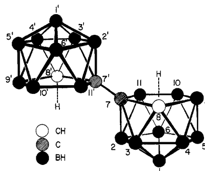
Figure 4.—The proposed structure and numbering system for the 7-(7'-7',8'-B 9 C 2 H 11 )-7,8-B 9 C 2 H 11 2- ion.
