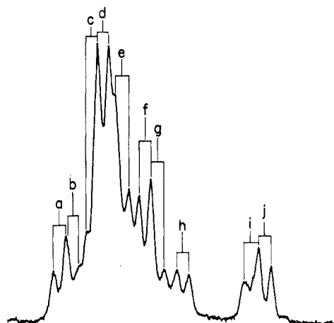
Figure 1.—An 80-MHz 11 B nmr spectrum of \text{Cs-7-(1'-1',2'-B}_{10}\text{C}_2\text{H}_{11})\text{-7,8-B}_9\text{C}_2\text{H}_{11} in acetone. Chemical shifts, relative to external \text{BF}_3\cdot\text{O}(\text{C}_2\text{H}_5)_2 (coupling constants, Hz): (a) +5.2 (158), (b) +7.2 (136), (c) +10.0 (138), (d) +11.8 (145), (e) +14.7 (161), (f) +18.1 (152), (g) +20.0 (152), (h) +23.7 (140), (i) +34.0 (140), (j) +36.3 (158).
