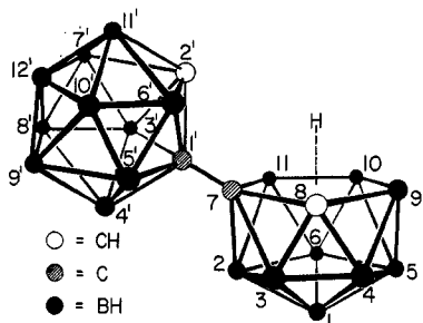
Figure 2.—The proposed structure and numbering system for the 7-(1'-1',2'-B 10 C 2 H 11 )-7,8-B 9 C 2 H 11 - ion.
