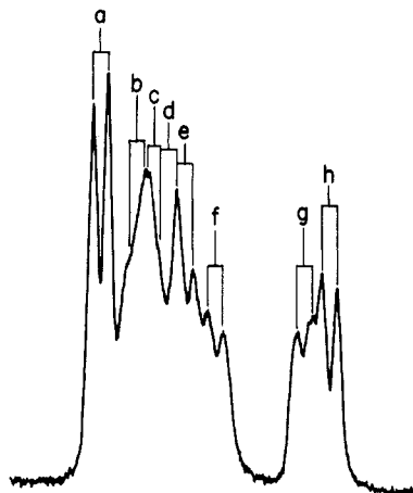
Figure 3.—An 80-MHz ^{11}\text{B} nmr spectrum of Cs 2 -7-(7'-7',8'-B 9 C 2 H 11 )-7,8-B 9 C 2 H 11 in acetone. Chemical shifts, relative to external BF 3 ·O(C 2 H 5 ) 2 (coupling constants, Hz): (a) +11.3 (150), (b) +15.4 (148), (c) +17.6 (129), (d) +18.9 (142), (e) +20.5 (137), (f) +24.0 (135), (g) +33.8 (148), (h) +36.4 (132).
