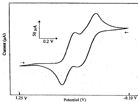
Fig. 2. Cyclic voltammogram for 3 at a 50 mV s -1 scan rate.
