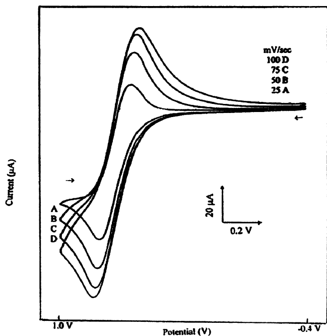
Fig. 1. Cyclic voltammogram for 1b at variable scan rates.
