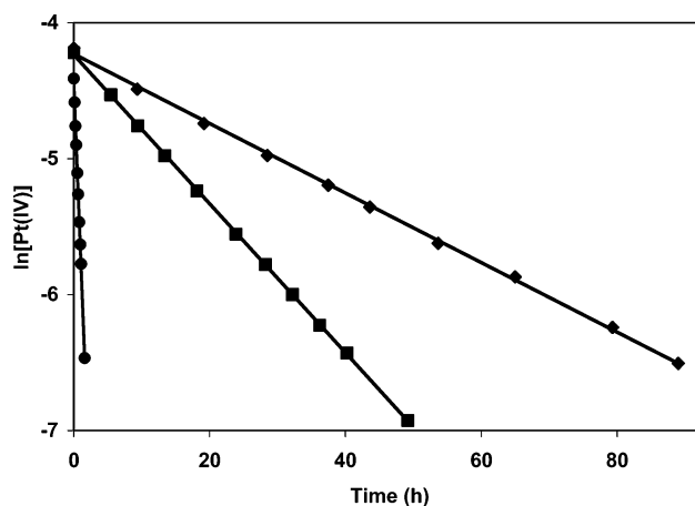
Figure 1. First-order kinetic plots of the disappearance of \text{L}_2\text{PtMe}_4 ( \bullet = \mathbf{1} , \blacklozenge = \mathbf{2} , \blacksquare = \mathbf{3} ) in \text{C}_6\text{D}_6 at 165 °C.
