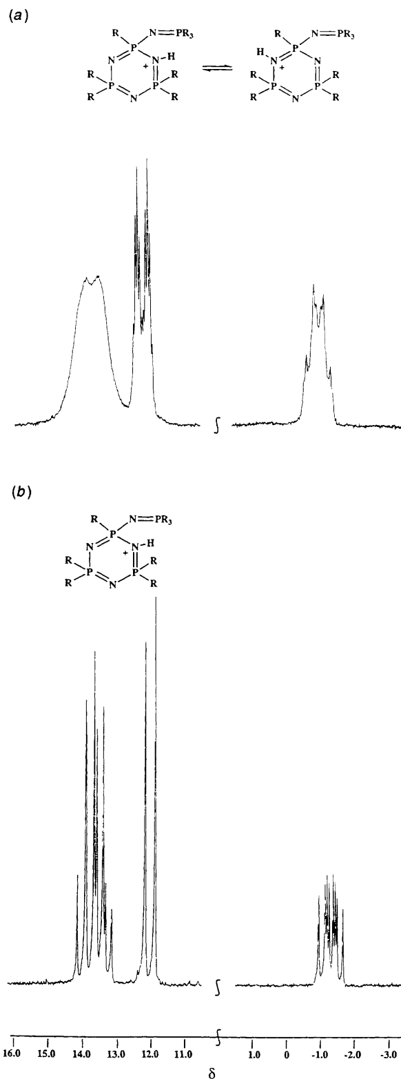
Fig. 5 Variable-temperature ^{31}P NMR spectra of trimer 7 in CD_3OD at (a) 20 and (b) -60^\circ C
