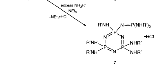
Scheme 2 R = Ph, R' = Pr
