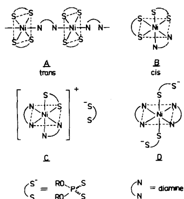
Figure 2. Suggested structures for the adducts.
