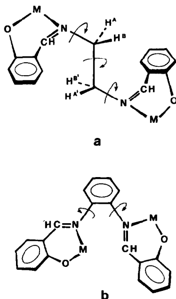
Fig. 1. Bonds rotation in salen (a) and saloph (b) bimetallic complexes.
