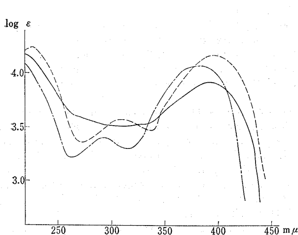
Fig. 2. UV Spectra of XIII, XVII, and XXV in EtOH.
