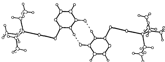
Fig. 2. Hydrogen bonding interactions in \text{Et}_3\text{PAu}(2\text{-TU}) .
