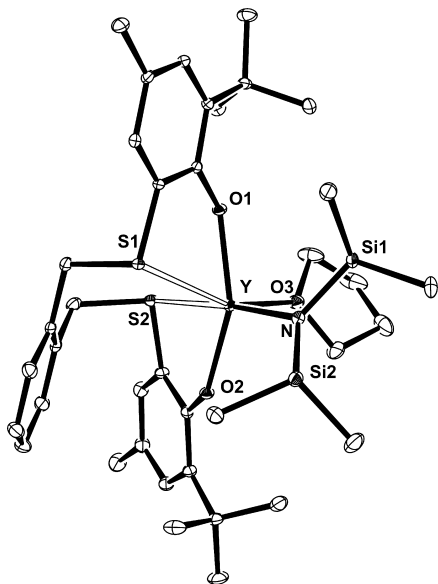
Figure 1. ORTEP diagram of the molecular structure of [Y(xytdmp)\{N(SiHMe_2)_2\}(THF)] ( 6b ). Thermal ellipsoids are drawn at the 30% probability level. Hydrogen atoms are omitted for clarity.
