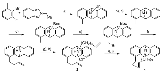
Scheme 1. Synthesis of (1S,4R)-(E)-1. Reagents and conditions: (a) Mg activated with \text{BrCH}_2\text{CH}_2\text{Br} , THF, reflux, 1.5 h, 76%; 6 (b) NBS, 1,4-dioxane/ \text{H}_2\text{O} , rt, 3 days; (c) quenching with KOH aq, 69% (overall yield for 2 steps); (d) (\text{Boc})_2\text{O} , \text{Et}_3\text{N} , MeOH, reflux, 1 h, 92%; (e) NBS, BPO, h\nu , \text{CCl}_4 , reflux, 3 h, 81%; (f) \text{CH}_2=\text{CHCH}_2\text{MgCl} , THF, reflux, 2 h, 69%; (g) \text{CH}_2=\text{CH}(\text{CH}_2)_3\text{Br} , \text{K}_2\text{CO}_3 , \text{CH}_3\text{CN} , reflux, 8 h; (h) quenching with HCl, \text{Et}_2\text{O} , 80% (overall yield for 2 steps); (i) the Grubbs' catalyst (the second generation), \text{CH}_2\text{Cl}_2 , reflux, 3 days, 75%; (j) separation on a Daicel Chiralcel OD column, 44%.
