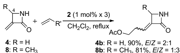
Scheme 2. The impact of C-4 branching on CM reactions.
