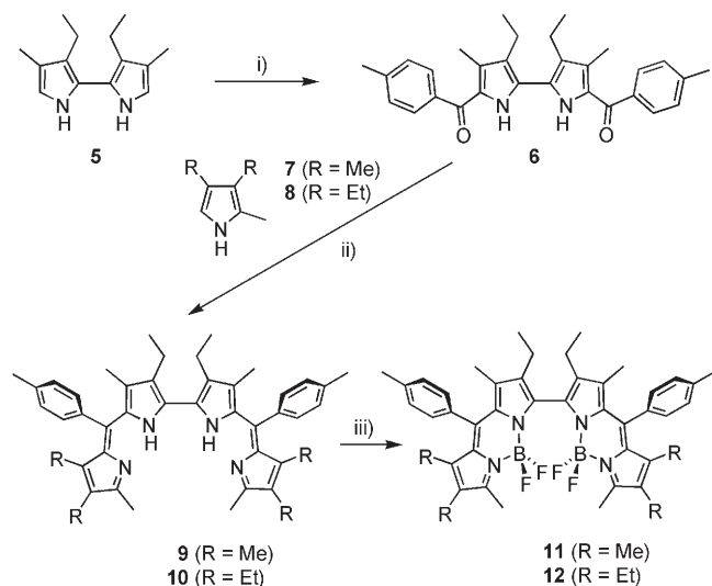
Scheme 2. Preparation of meso -aryl-substituted bisBODIPYs 11 and 12 . i) N -4-Methylbenzoylmorpholine, \text{POCl}_3 , 1,2-dichloroethane, 48%; ii) \text{POCl}_3 , \Delta , 70% ( 7 ) and 67% ( 8 ); iii) \text{BF}_3 \cdot \text{Et}_2\text{O} , 2,6-lutidine, diethyl ether, 65%.
