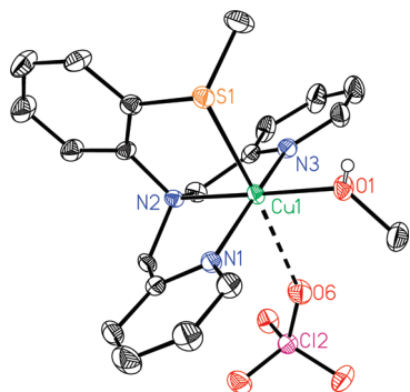
Figure 5. Molecular structure of a cationic portion \{[(L^{ASM})Cu^{II}(CH_3OH)](ClO_4)\}^+ ( 1e ) ClO_4^- from X-ray crystallographic analysis. A non-coordinated perchlorate counteranion and hydrogen atoms (except that for the coordinated MeOH group) have been omitted for clarity.
