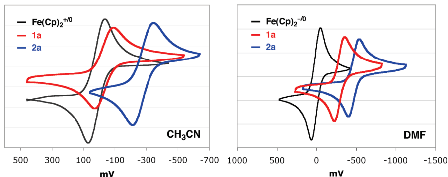
Figure 4. Cyclic voltammograms of [(L^{ASM})Cu^I]^+ ( 1a , red) and [(L^{ESF})Cu^I]^+ ( 2a , blue) measured in CH_3CN (left) and DMF (right) under Ar. E_{1/2} values reported (Table 3) are versus [Fe(Cp)_2]^{+/0} (black) measured as an external standard under the same conditions.
