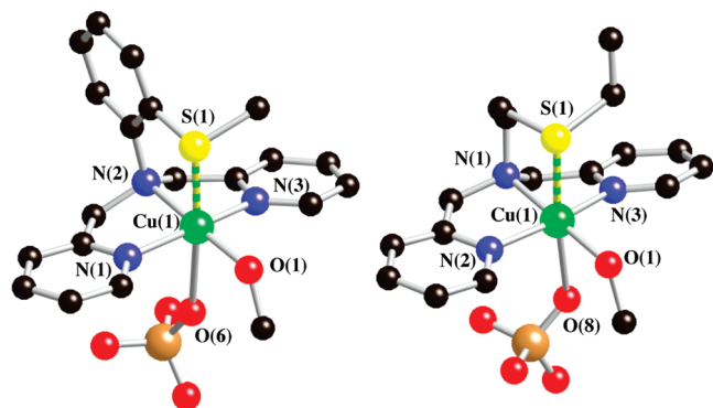
Figure 6. Molecular structure comparison between isolated cations of \{[(L^{ASM})Cu^{II}(CH_3OH)](ClO_4)\}^+ ( 1e ) ClO_4^- and \{[(L^{ESF})Cu^{II}(CH_3OH)](ClO_4)\}^+ ( 2c ) ClO_4^- derived from X-ray crystallographic analysis. Hydrogen atoms are omitted for clarity.
