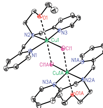
Figure 8. X-ray structure of a cationic portion [(L^{EOE})Cu^{II}(Cl)]^{2+} ( 3c ). The B(C_6F_5)_4^{-} counteranion and hydrogen atoms are omitted from the ORTEP view for clarity.
