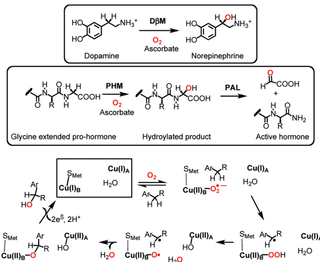
Figure 1. Enzymatic hydroxylations of substrates by \text{D}\beta\text{M} and PHM (top and middle) and one proposed mechanism of PHM and \text{D}\beta\text{M} (bottom). See text.
