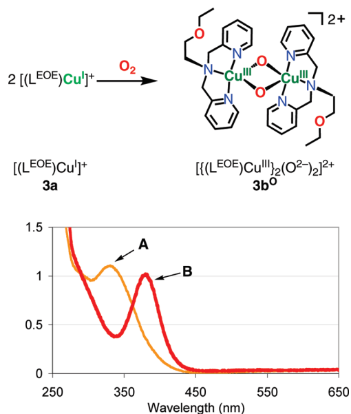
Figure 11. Low-temperature UV-vis spectra of A: [(L^{EOE})Cu^I]^+ ( 3a ) absorption at 329 nm, 5,000\text{ M}^{-1}\text{ cm}^{-1} ; B: [(L^{EOE})Cu^{III}]_2(O_2^{2-})_2^{2+} ( 3b O ) absorption 380 nm ( 10,000\text{ M}^{-1}\text{ cm}^{-1} ) in THF at -94\text{ }^\circ\text{C} .
