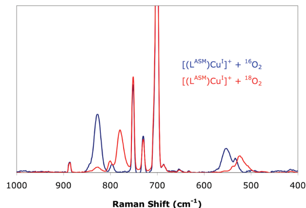
Figure 10. Resonance Raman spectra of [\{(\text{L}^{\text{ASM}})\text{Cu}^{\text{II}}\}_2(\text{O}_2^{2-})]^{2+} ( 1b P ) in THF at 77 K (blue spectrum denotes 16 O 2 , red spectrum denotes 18 O 2 . \lambda_{\text{ex}} = 568 nm. \nu(\text{O}-\text{O}) = 828 cm -1 ( \Delta(^{18}\text{O}_2) = 48 ), \nu_{\text{sym}}(\text{Cu}-\text{O}) = 547 cm -1 ( \Delta(^{18}\text{O}_2) = 23 ) and \nu_{\text{asym}}(\text{Cu}-\text{O}) = 497 cm -1 ( \Delta(^{18}\text{O}_2) = 22 ).
