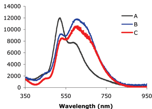
Figure 12. Low-temperature UV-vis spectra: A (black), [(tmpa)Cu^{II}]_2(O_2^{2-})_2^{2+} ; B (blue), [(L^{ESE})Cu^{II}]_2(O_2^{2-})_2^{2+} ( 2b P ); and C (red), [(L^{ASM})Cu^{II}]_2(O_2^{2-})_2^{2+} ( 1b P ).
