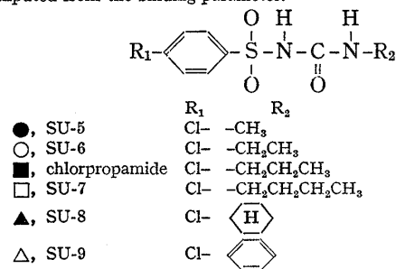
Fig. 2. Scatchard Plots for the Binding of Sulfonylurea Related Compounds ( R_1 : \text{Cl} ) to Bovine Serum Albumin at pH 7.4 and 30^\circ
