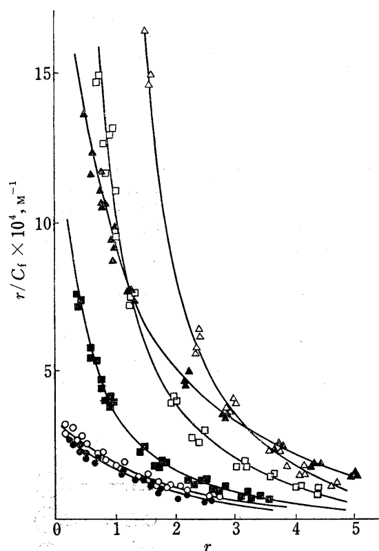
Fig. 2. Scatchard Plots for the Binding of Sulfonylurea Related Compounds ( R_1 : \text{Cl} ) to Bovine Serum Albumin at pH 7.4 and 30^\circ
