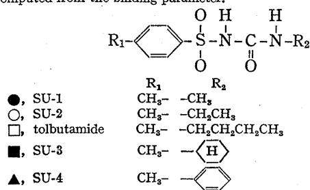
Fig. 1. Scatchard Plots for the Binding of Sulfonylurea Related Compounds ( R_1 : \text{CH}_3 ) to Bovine Serum Albumin at pH 7.4 and 30^\circ
