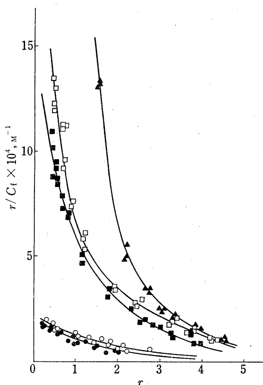
Fig. 1. Scatchard Plots for the Binding of Sulfonylurea Related Compounds ( R_1 : \text{CH}_3 ) to Bovine Serum Albumin at pH 7.4 and 30^\circ
