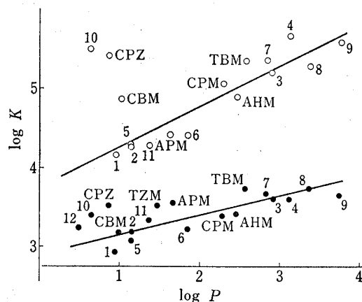
Fig. 4. Relationship between Binding Constants and Octanol/Water Partition Coefficient of Sulfonylurea Related Compounds at pH 7.4 and 30^\circ
