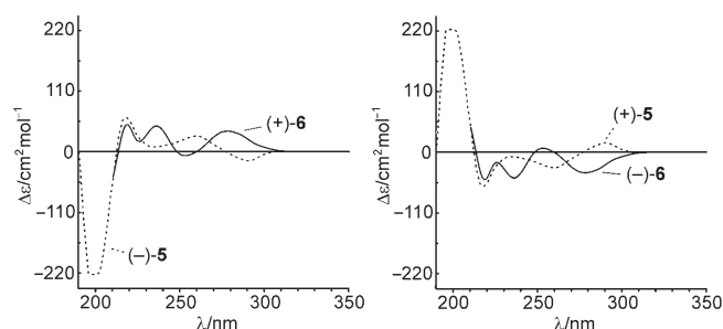
Figure 5. CD spectra of the two enantiomers of 5 (----) and 6 (—), in \text{CH}_3\text{CN} , c = 4 \times 10^{-5} \text{ mol L}^{-1} .
