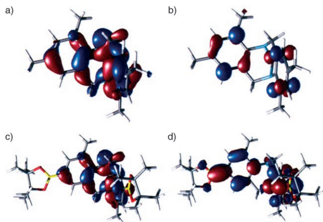
Figure 11. Calculated HOMOs (a and c) and LUMOs (b and d) of 6 (bottom) and 7 (top) obtained from B3LYP/6-31G* calculations.
