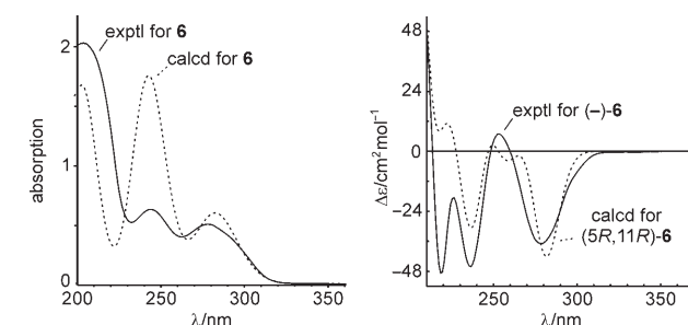
Figure 7. Calculated (TD B3LYP/6-31G*/B3LYP/6-31G*; ----) and experimental (—) UV spectra of 6 and corresponding experimental CD spectra of (-)\text{-6} (—) and calculated CD spectra of (5R,11R)\text{-6} .
