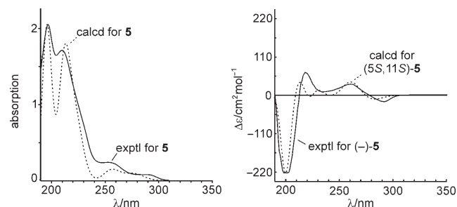
Figure 6. Calculated (B3LYP/6-31G*; ----) and experimental (—) UV spectra of 5 and corresponding experimental CD spectra of (-)\text{-5} (—) and calculated CD spectra of (5S,11S)\text{-5} .
