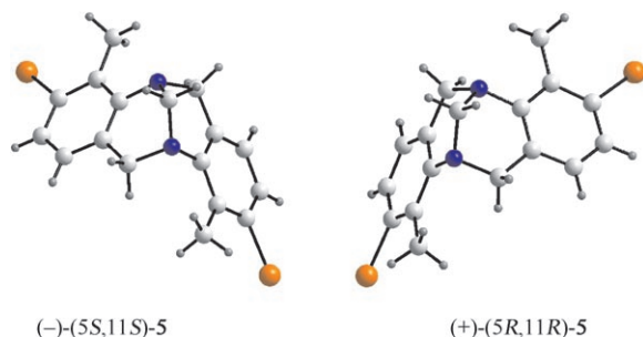
Figure 4. Crystal structures of (-)-(5S,11S)\text{-5} and (+)-(5R,11R)\text{-5} as determined by X-ray diffraction analysis.
