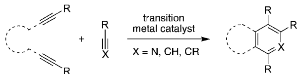
Scheme 1. General [2+2+2] Cyclotrimerization Reaction to (Fused) Benzenes and Pyridines
