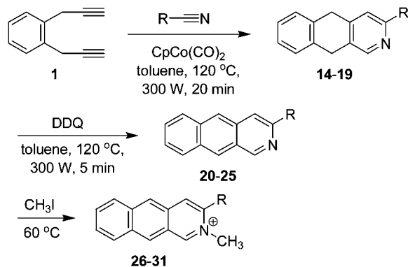
Scheme 3. Azanthracene Synthesis via [2+2+2] Cyclotrimerization
