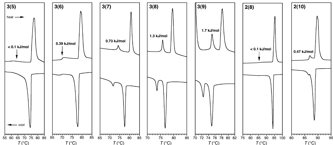
Figure 5. Partial DSC traces of compounds 3(5)–9 , 2(8) , and 2(10) showing the SmC–SmA and SmA–I phase transitions on heating and cooling at 5 K/min, and the enthalpy change for the SmA–SmC phase transition \Delta H_{AC} in kJ/mol.
