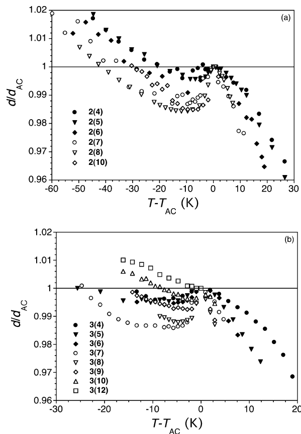
Figure 7. Relative smectic layer spacing d/d_{AC} versus reduced temperature T - T_{AC} for (a) compounds 2 ( n ) and (b) compounds 3 ( n ). The measurements were performed on heating from the crystalline phase for all compounds except 3 (9) and 3 (10), which were performed on cooling from just below the clearing point due to the narrow SmC temperature ranges. The data for 2 (8) are from ref 17.
