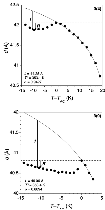
Figure 9. Smectic layer spacing d versus reduced temperature T - T_{AC} for compounds 3 (4) and 3 (9). The dashed lines show the layer spacing at the SmA–SmC transition. The solid lines represent the fits to eq 6 for the data points at T - T_{AC} \geq 0 . The arrows indicate the difference in layer spacing for calculating the R and f reduction factors.
