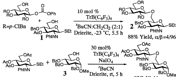
Scheme 1. \text{TrB}(\text{C}_6\text{F}_5)_4 catalyzed glycosylation reactions.
