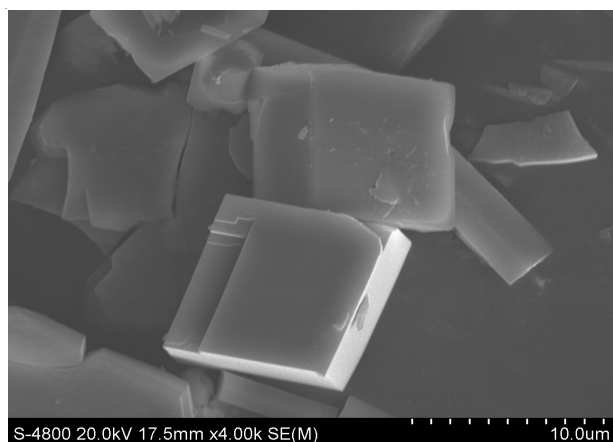
(a) SEM photograph of calcium carbonate sample from blank solution
