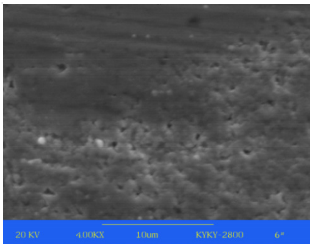
(c) SEM image of corrosive test piece from the solution with polyepoxysuccinic acid
