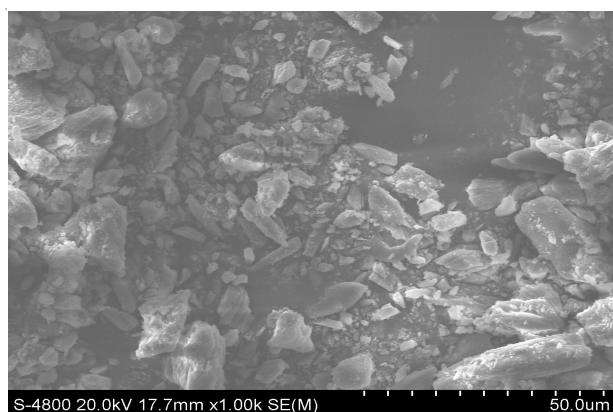
(b) SEM photograph of calcium carbonate sample from the solution with 1 mg L -1 polyepoxysuccinic acid derivative
