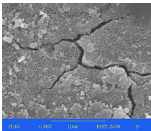
(b) SEM image of corrosive test piece from blank water
