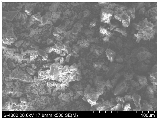
(c) SEM photograph of calcium carbonate sample from the solution with 2 mg L -1 polyepoxysuccinic acid derivative
