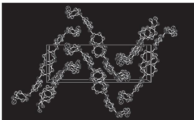
Fig. 3 Packing diagram of the molecule viewed down the a -axis.
