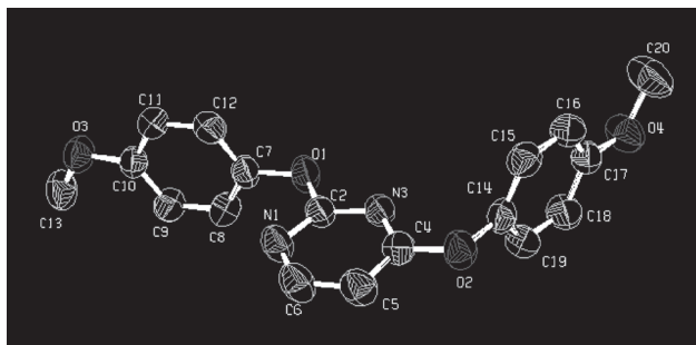
Fig. 2 Molecular structure showing 50% probability displacement ellipsoids.
