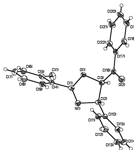
Figure 1. ORTEP plots of 4i ( \text{C}_{22}\text{H}_{16}\text{ClNO}_2 ).
