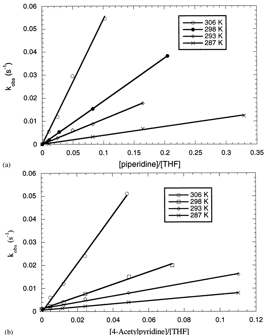
Fig. 4. (a) A plot of k_{\text{obs}} versus [\text{piperidine}]/[\text{THF}] at four temperatures for the reaction of \text{CpMn}(\text{CO})_2(\text{THF}) with piperidine in THF solvent. (b) Plot of k_{\text{obs}} versus [\text{4-acetylpyridine}]/[\text{THF}] for the reaction of the Mn complex with 4-acetylpyridine in THF solvent.
