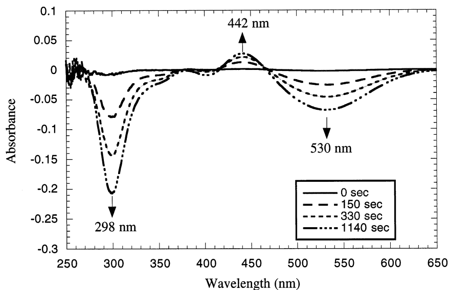
Fig. 3. Difference spectra showing growth of the \text{CpMn(CO)}_2(\text{pip}) complex at 442 nm and decay of the \text{CpMn(CO)}_2(\text{THF}) complex at 298 and 530 nm.
